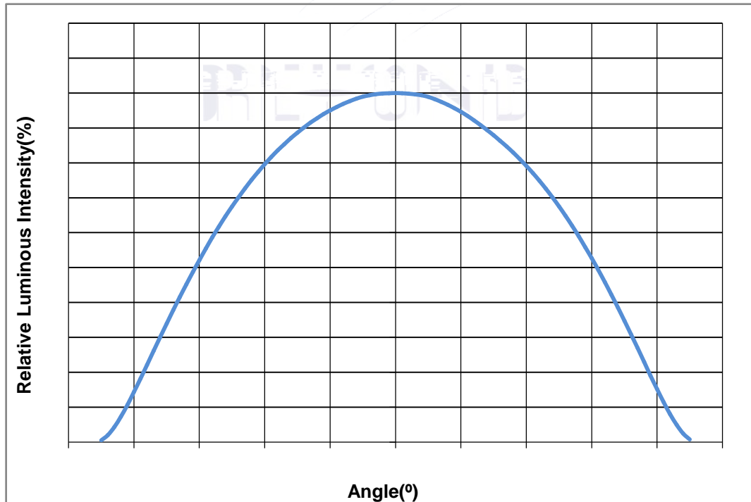
Fig. 1-12 Radiation diagram
