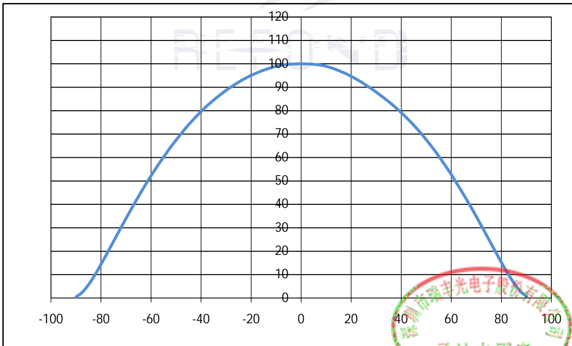
Fig. 1-12 Radiation diagram
