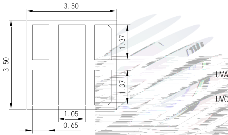
Fig.1-3 Bottom view
