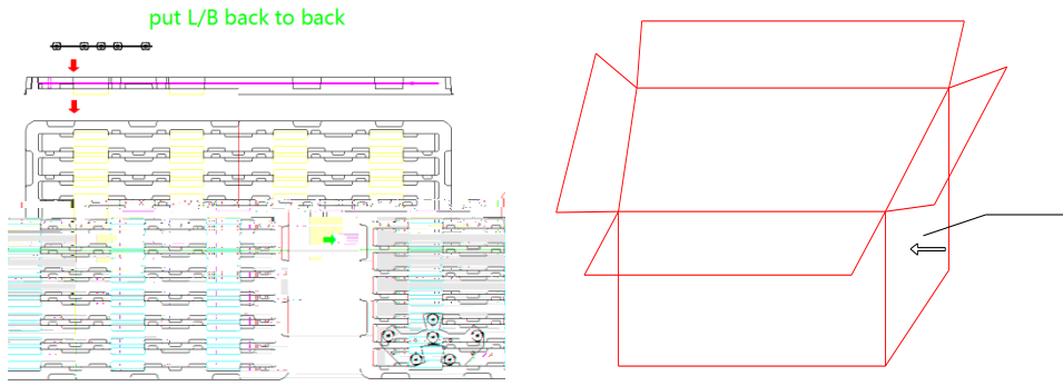
Fig 8-1Package Diagram /
